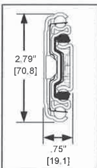
Model 7957 Handed lever disconnect
